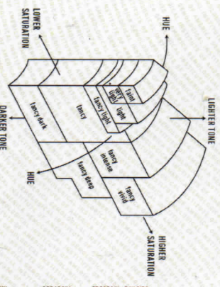
Illustration of GIA fancy color grade interrelationships
