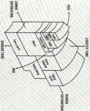
Illustration of GIA fancy color grade interrelationships
